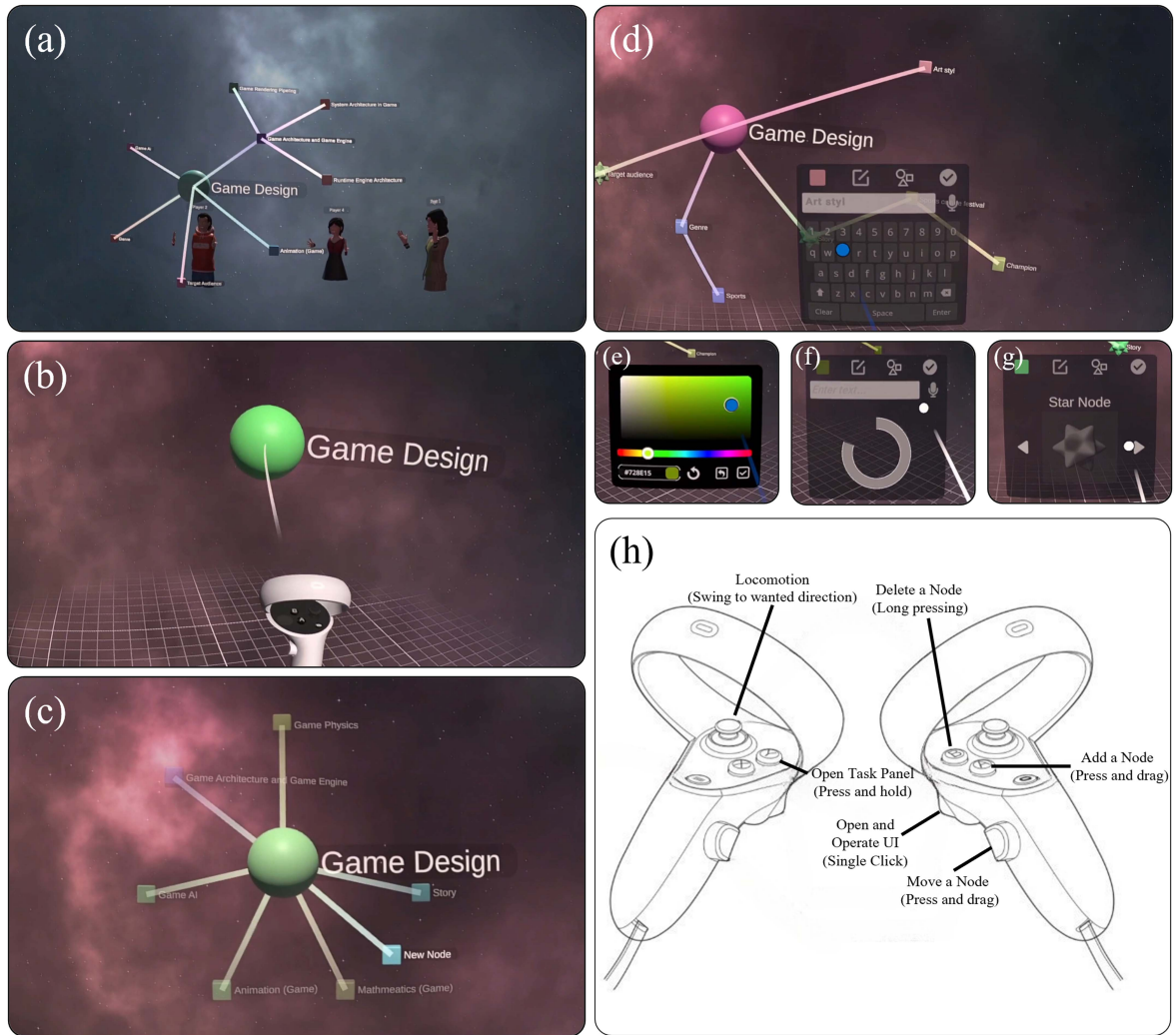
Fig. 1. Overview of our KG-driven MM editor in an edu-metaverse setting. (a) Players collaborating on an MM. (b) Root node and interaction ray between the controller and a target node. (c) Semitransparent dummy nodes for recommendations. (d)–(g) UI features: the text editor, color picker, voice-to-text, and shape selector. (h) Buttons and triggers bindings on controllers to operate in the system.
