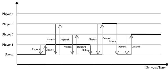
Fig. 2. Node control authority management of our system in a timeline chart: The virtual room allocates the authority in the FIFS manner. The clients send requests to the room applying for authority and will be rejected if other players take over the node.
